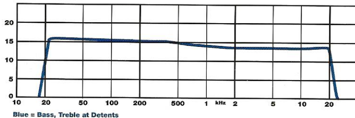
ORION ELECTRONICS Bass & Treble CW, CCW
